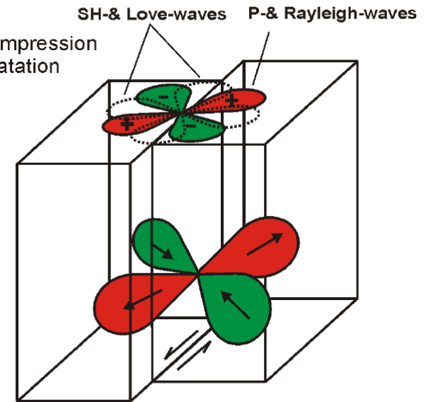
Earthquake (strike-slip)
