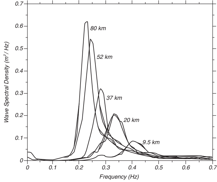
Figure 16.9 Wave spectra of a developing sea for different fetches measured at JONSWAP. After Hasselmann et al. (1973).
