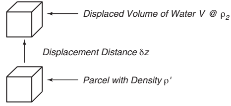
Figure 8.5 Sketch for calculating static stability and stability frequency.
