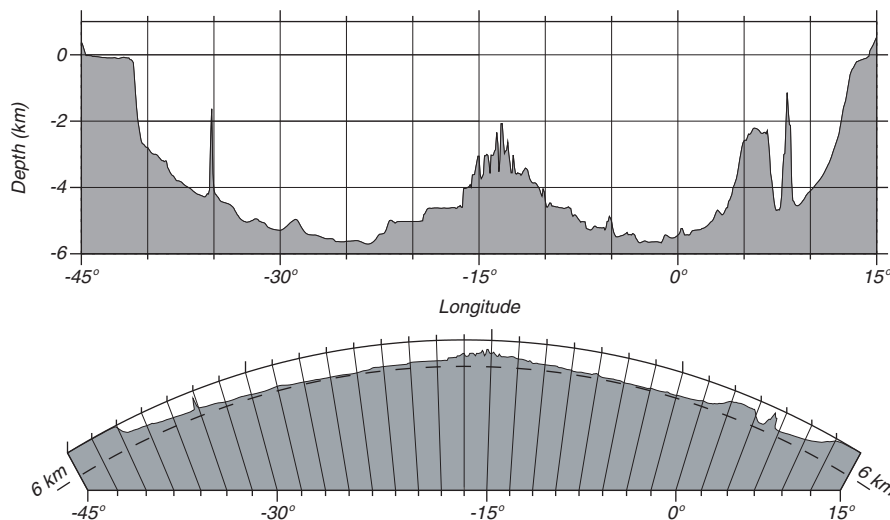
Figure 3.4 Cross-section of the south Atlantic along 25°S showing the continental shelf offshore of South America, a seamount near 35°W, the mid-Atlantic Ridge near 14°W, the Walvis Ridge near 6°E, and the narrow continental shelf off South Africa. Upper Vertical exaggeration of 180:1. Lower Vertical exaggeration of 30:1. If shown with true aspect ratio, the plot would be the thickness of the line at the sea surface in the lower plot.
