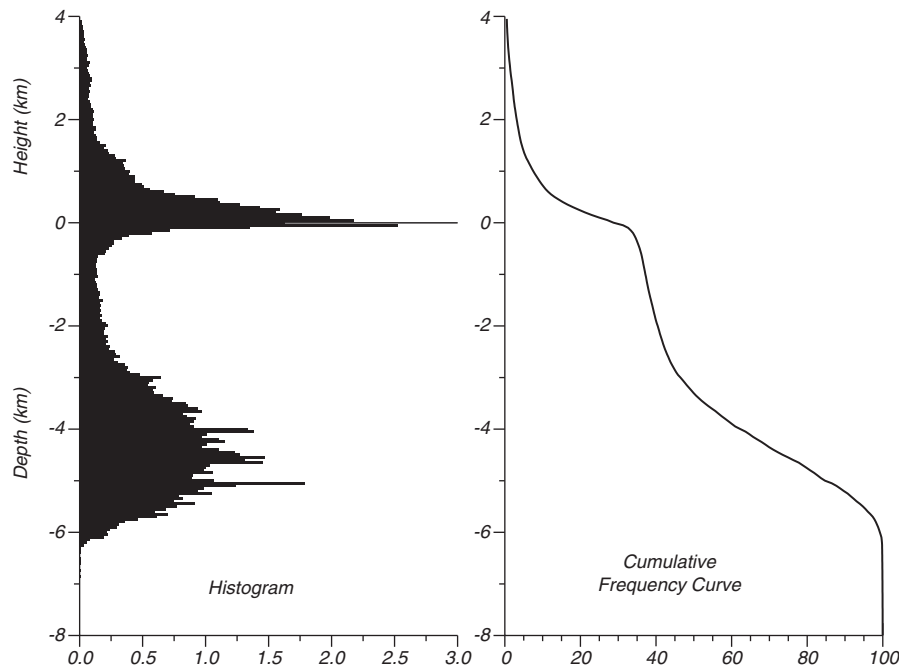
Figure 3.5 Left Histogram of elevations of land and depth of the sea floor as percentage of area of Earth, in 50 m intervals showing the clear distinction between continents and sea floor. Right Cumulative frequency curve of height, the hypsographic curve. The curves are calculated from the ETOPO 30' data set.
