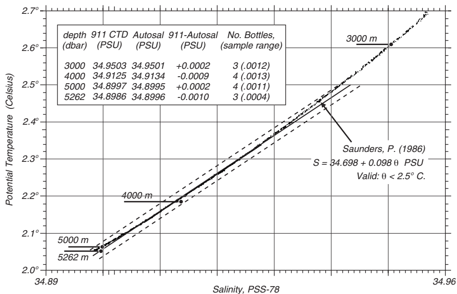
Figure 6.15. Results from a test of the Sea-Bird Electronics 911 Plus CTD in the North Atlantic Deep Water in 1992. Data were collected at 43.17^\circ \text{N} and 14.08^\circ \text{W} from the R/V Poseidon. From Sea-Bird Electronics (1992).
