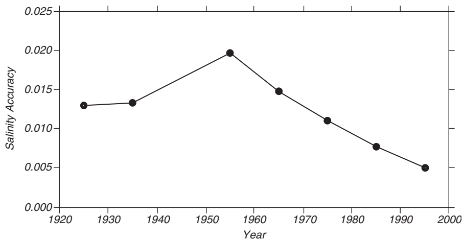
Figure 6.14. Standard deviation of salinity measurements at depths below 1500 m in the south Atlantic from 1920 to 1993. Each point is the average of data collected for the decade centered on the point. The value for 1995 is an estimate of the accuracy of recent measurements. From table 1 of Gouretski and Jancke (1995).
