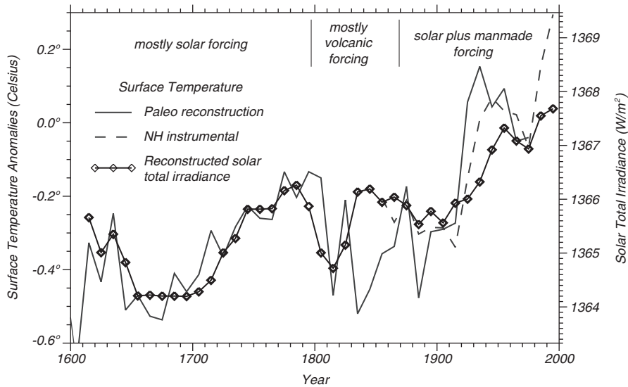
Figure 5.13 Changes in solar constant (total solar irradiance) and global mean temperature of earth's surface over the past 400 years. Except for a period of enhanced volcanic activity in the early 19th century, surface temperature is well correlated with solar variability. After Lean, personal communication.
